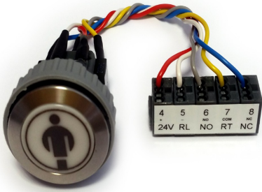
Ruf-Taster TA-099-310-61 (VRT)
